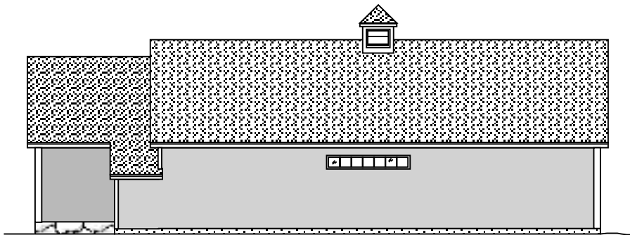
left elevation
