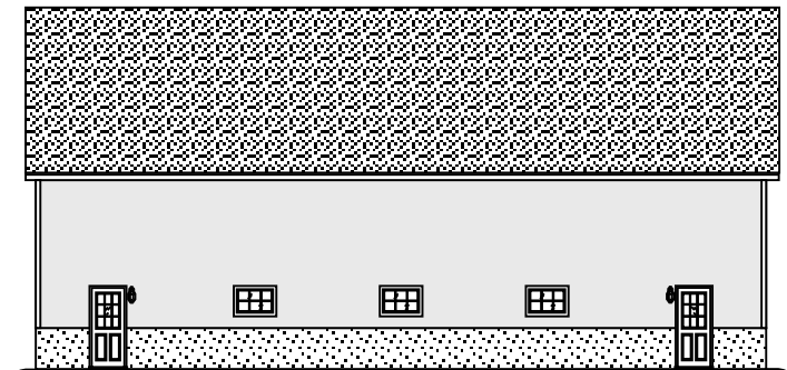
left elevation
