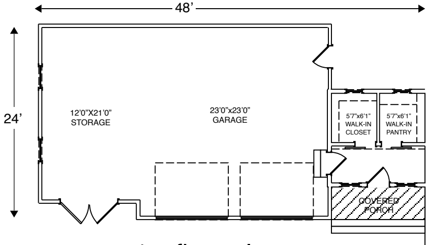
1st floor plan
