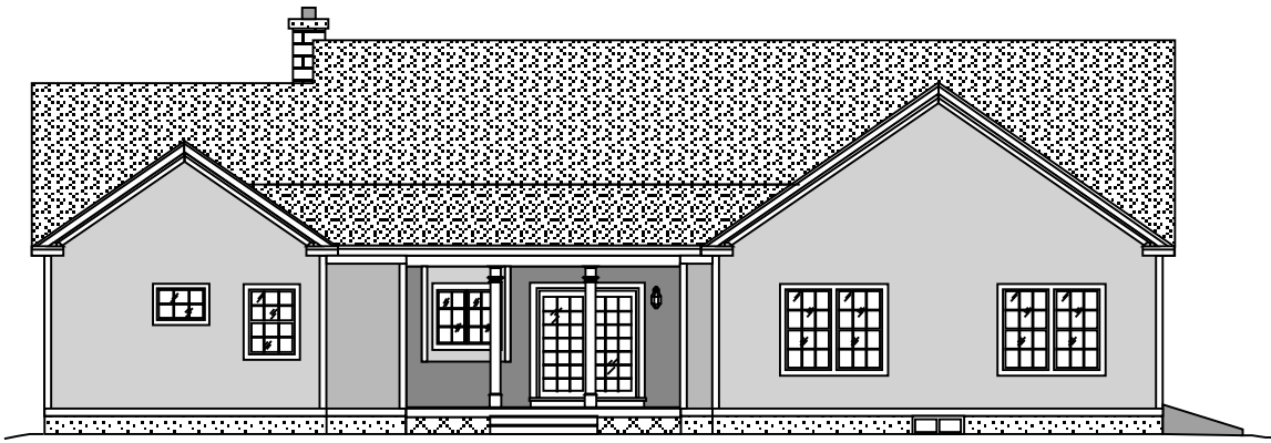
rear elevation
