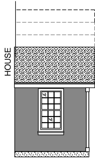
rear elevation
