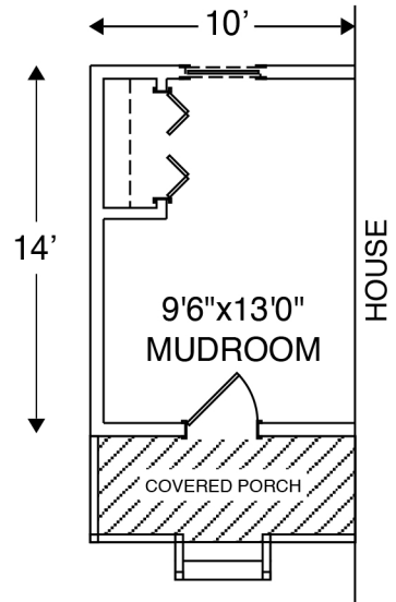
floor plan
