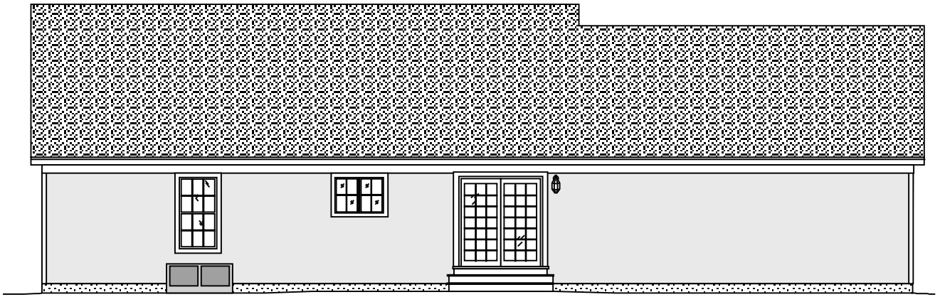
rear elevation
