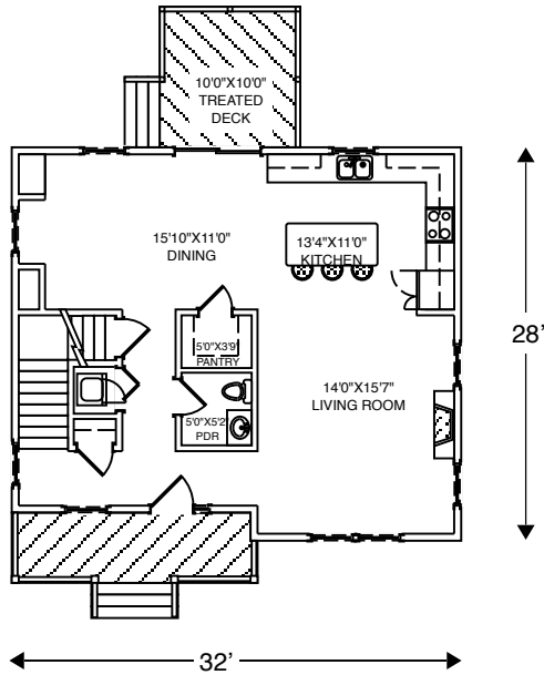
1st FLOOR PLAN 860 sq ft
