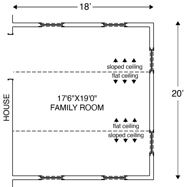
floor plan
