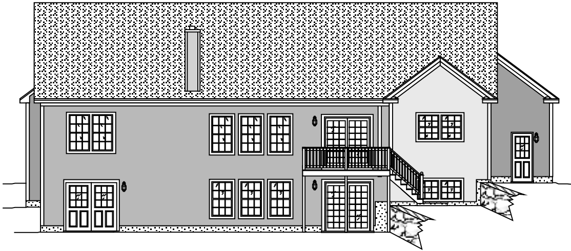
rear elevation
