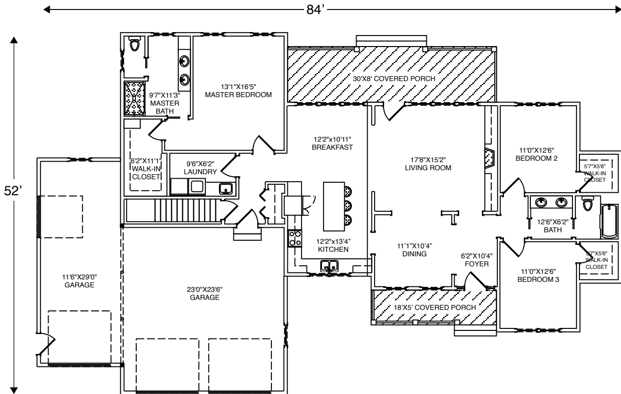
1st FLOOR PLAN ← 1971 sq ft
