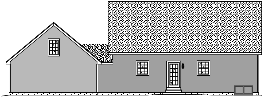
rear elevation
