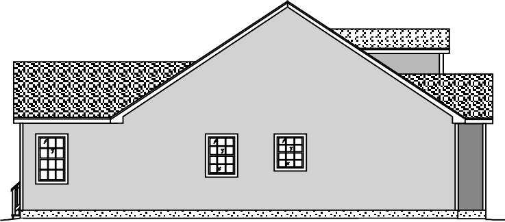
left elevation
