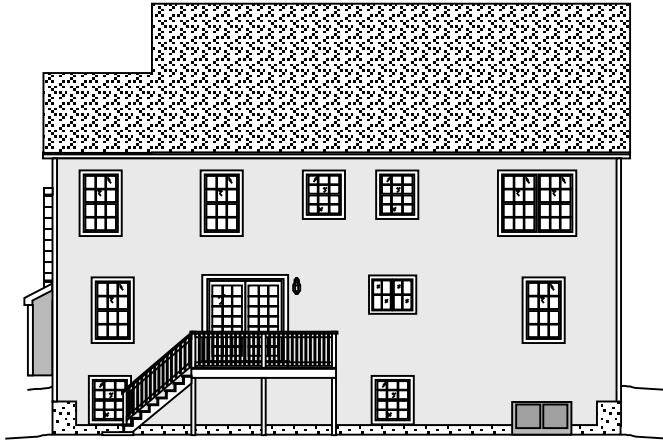
rear elevation
