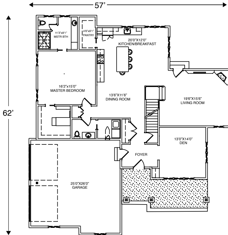
1st FLOOR PLAN 1662 sq ft
