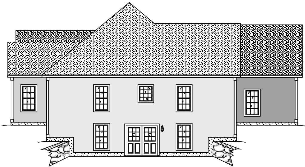
left elevation
