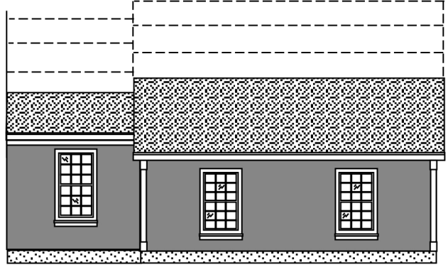
rear elevation
