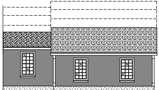
rear elevation
