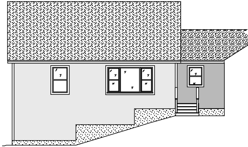
rear elevation
