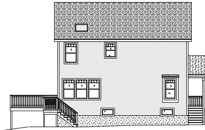
left elevation
