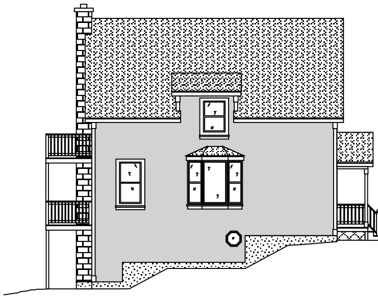
left elevation
