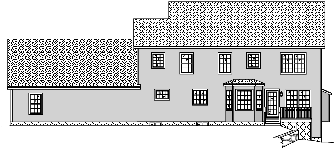
rear elevation
