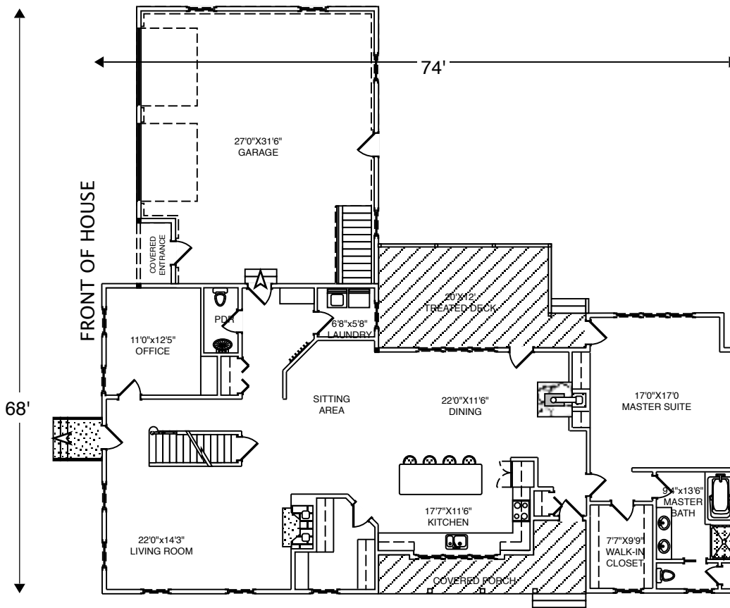
1st FLOOR PLAN 2283 sq ft
