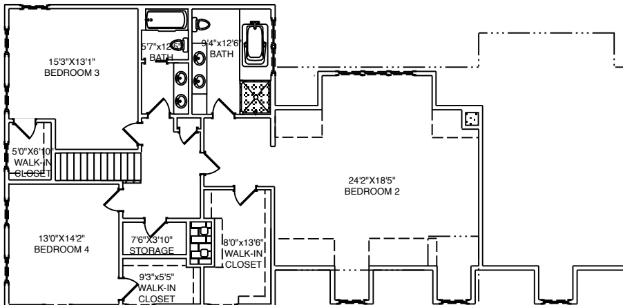
2nd FLOOR PLAN 1720 sq ft
