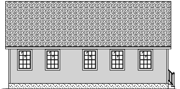
left elevation
