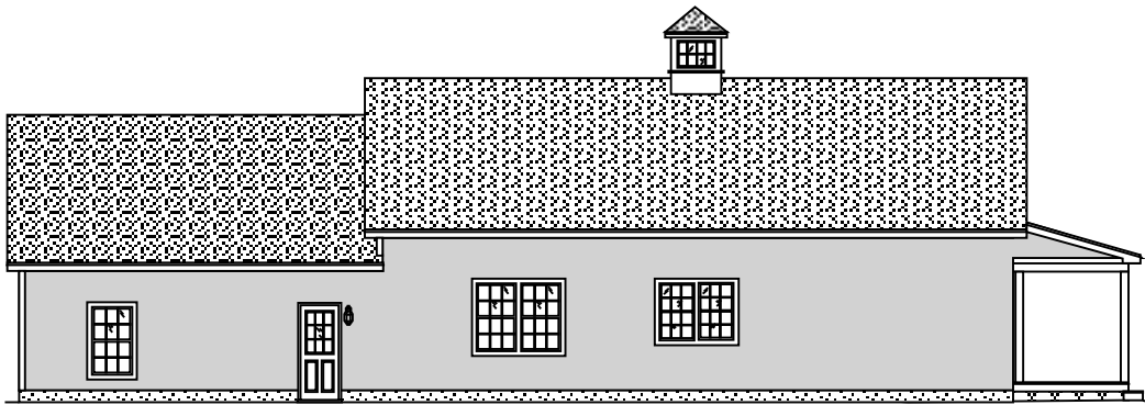
left elevation
