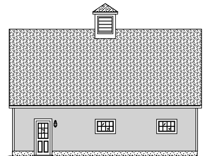
left elevation
