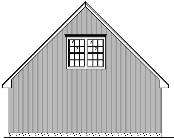
rear elevation
