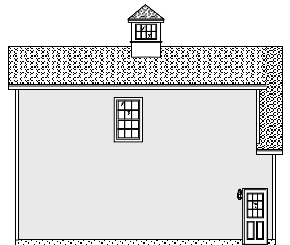
left elevation
